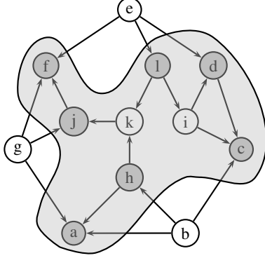
Figure 1. A minimum vertex cover (vertices in gray) and the cover given by a permutation \pi of the vertices in the graph (vertices inside the shaded area). The orientation of the edges is determined by \pi .
